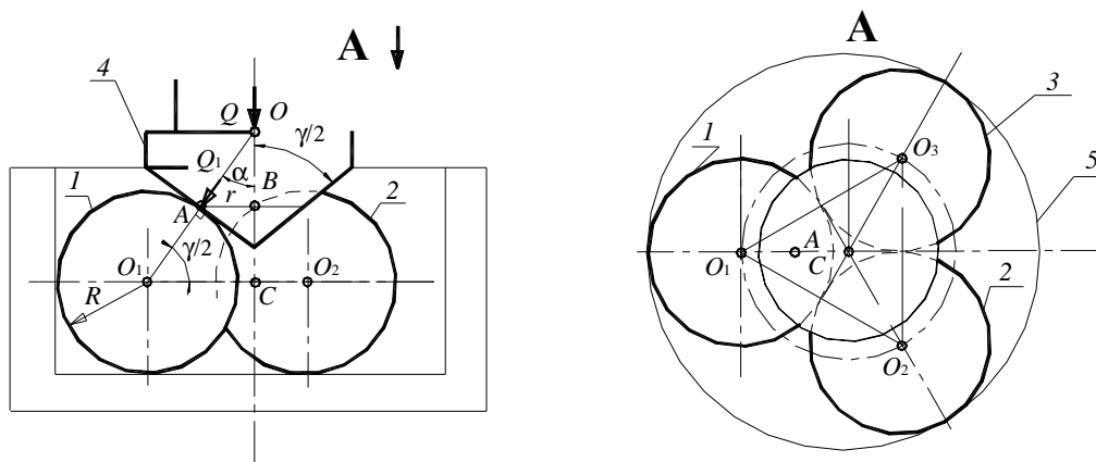
Fig. 1 - Diagram "cone - three balls"
